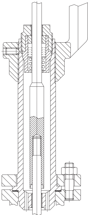
Fig. 3 · Detailed drawing of the insulating section
