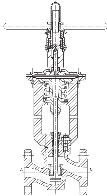
Fig. 4 · Type 3351-1 Pneumatic On/off Valve with handwheel
