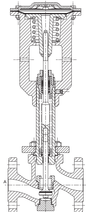
Fig. 5 · Type 3351-1 Pneumatic On/off Valve version with bellows seal
