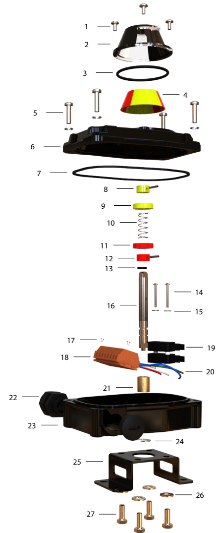
A250 PSM-PSP Standard Switch Boxes
